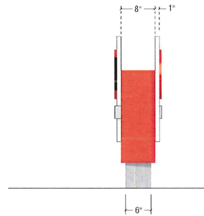
2 End View — Fabrication Scale: 1:4
