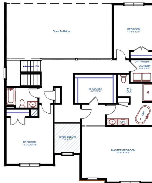
Second Floor - Deluxe Bathroom Plan
