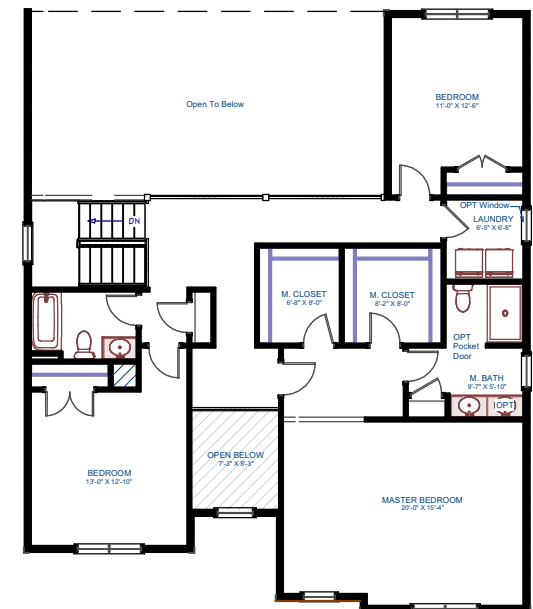
Second Floor - Standard Plan
